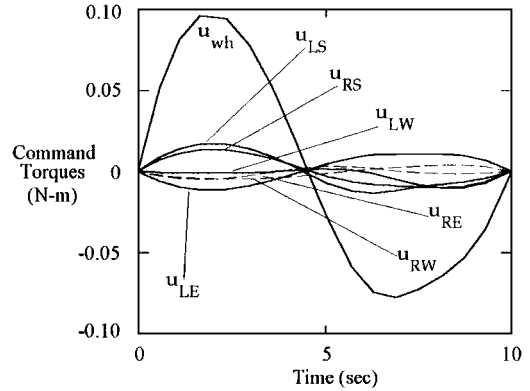
Fig. 7 Nominal fifth-order command torques.
