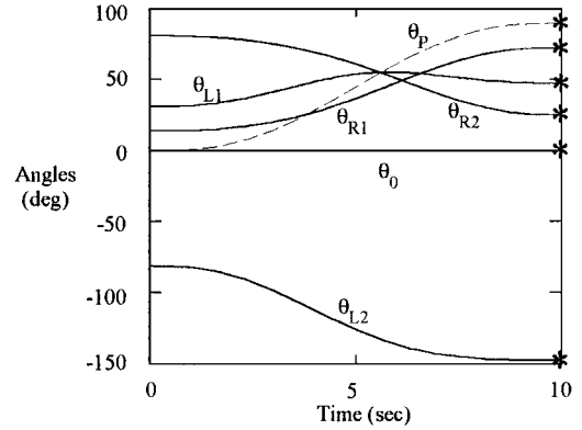
Fig. 6 Nominal fifth-order angles.
